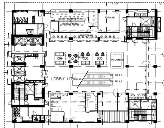
Layout Plan
