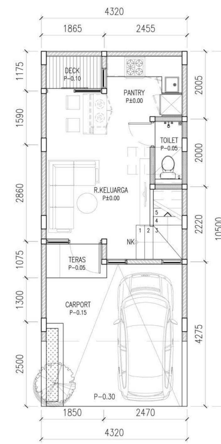
DENAH LANTAI 1
