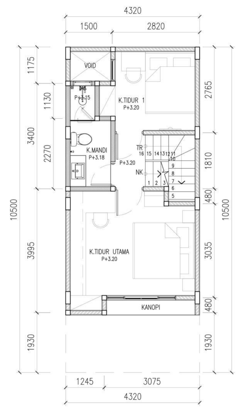
DENAH LANTAI 2
