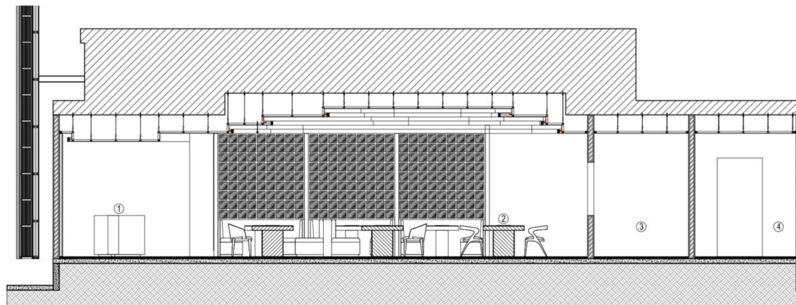
SECTION B-B
