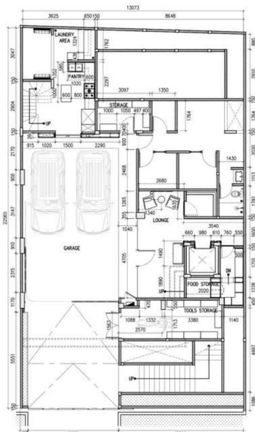
Semi-Basement Floor Plan
